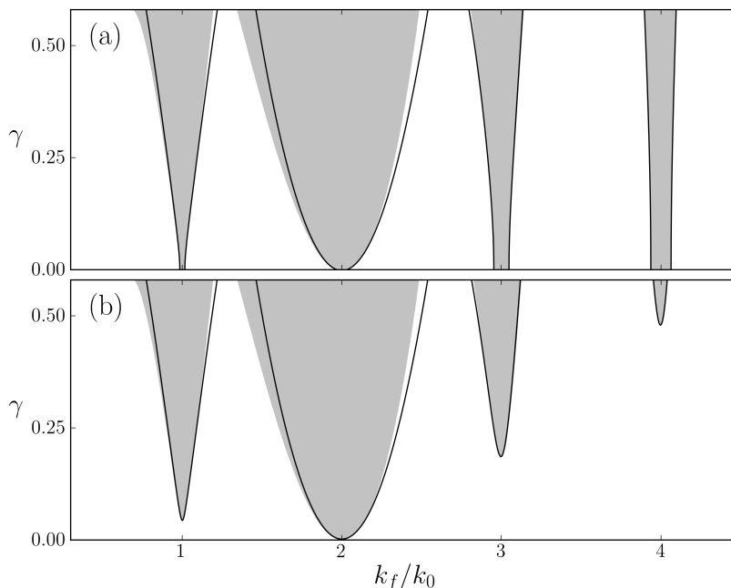
Figure 3.1: Existence domains of resonant stripe solutions of Equation (3.1), (a) above ( \epsilon > 0 ), and (b) below ( \epsilon < 0 ) the pattern forming instability. The shaded regions indicate the range of resonant solutions computed from stationary solutions of Equation (3.1), and the solid curves show the region boundary approximations (Equations. (3.18) and (3.21)) based on the amplitude equation approach. The agreement for the lower resonances is very good for sufficiently small \gamma values, and for the higher resonances it remains surprisingly good, even for large \gamma values. Parameters: k_0 = 1 and (a) \epsilon = 0.001 , (b) \epsilon = -0.001 .
