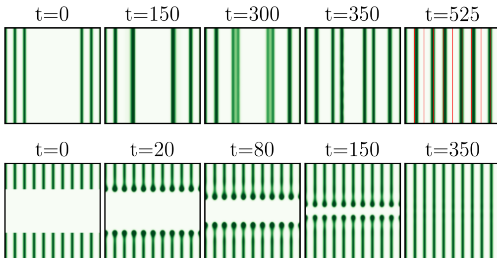
Figure 5.14: Tangential and normal fronts of stripe pattern and bare soil solutions, for p = 0.95 . While in the case of normal fronts the steady state is a 1 : 1 wavenumber locked stripe pattern, in the case of tangential fronts, the steady state is a stripe pattern with no clear periodicity.
