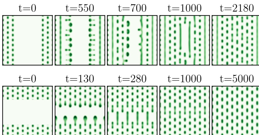
Figure 5.12: Tangential and normal fronts of rectangular and bare soil solutions, for p = 0.89 . In both cases the vegetation invades the bare soil region, and the system converges to the rectangular pattern (albeit with some defects and stripe regions in the case of tangential fronts).
