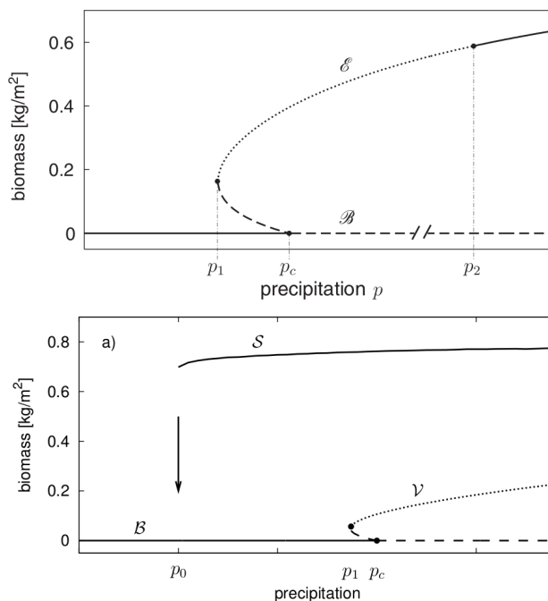
Figure 2.9: Bifurcation graph of uniform solutions of Equations (2.26). The graph on the top shows two branches of uniform solutions, the bare soil solution \mathcal{B} and the uniform cover solution \mathcal{E} . The graph on the bottom shows an additional branch \mathcal{S} , that corresponds to a spot-pattern solution. Full lines denote stability, while broken lines indicate instability. The graph on the top was taken from [51], and the one on the bottom was taken from [72].
