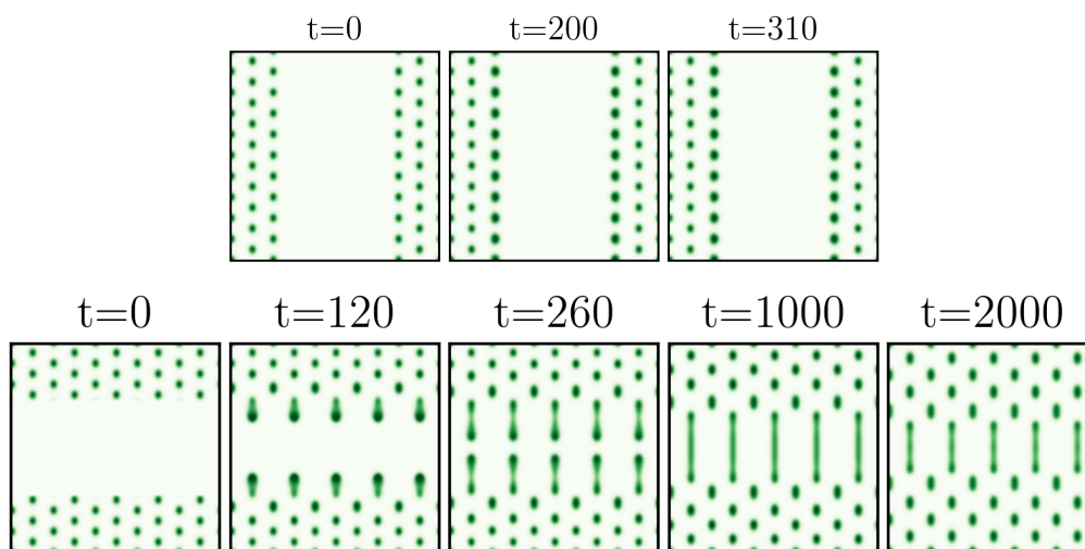
Figure 5.10: Tangential and normal fronts of rectangular and bare soil solutions, for p = 0.80 . The forcing varies in the x (horizontal) direction. The panels on the top indicate that the tangential front is static, while the panels on the bottom show that vegetation can invade the bare soil solution from a normal front.
