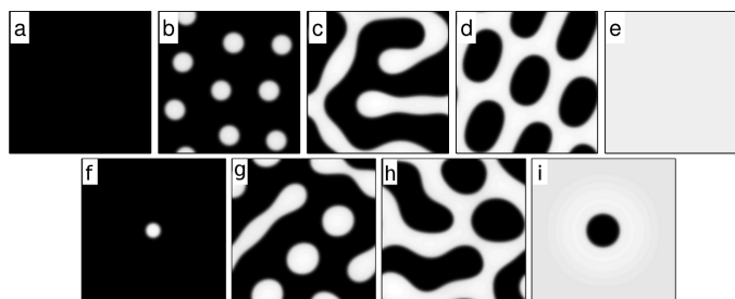
Figure 2.10: Panels ‘a’ through ‘e’ show five kinds of solutions of (2.26) for increasing precipitation rate values, from left to right: bare soil, spots, stripes, gaps, and uniform cover. Panels ‘f’ through ‘i’ show combinations of neighboring bistable solutions. Figure adapted from [73].
