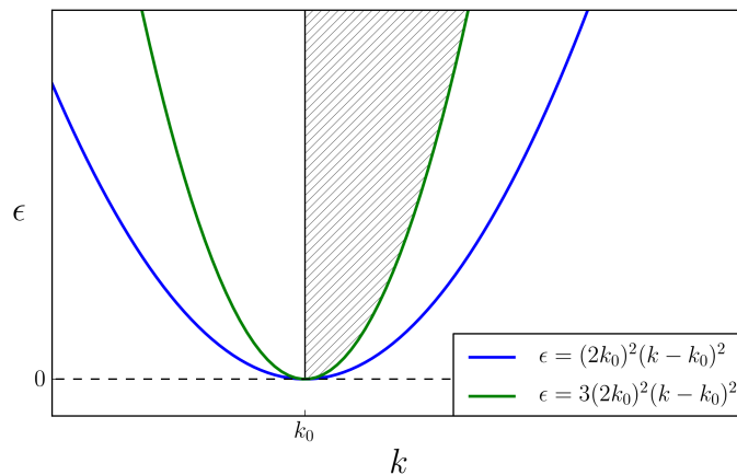
Figure 2.5: Parameter space \epsilon versus k . The shaded area denotes the region where stripe solutions of Equation (2.1) are stable to both longitudinal (Eckhaus) and transverse (zigzag) instabilities.
