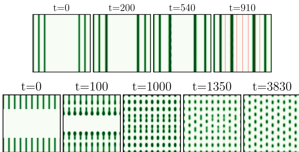
Figure 5.13: Tangential and normal fronts of stripe pattern and bare soil solutions, for p = 0.89 . In the case of tangential fronts, the stripes migrate and the steady state consists of a stripe pattern with no clear periodicity. When the front is normal, the steady state is a rectangular pattern.
