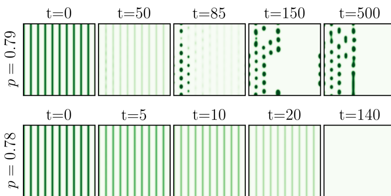
Figure 5.9: The evolution of the biomass for a stripe pattern for precipitation values p = 0.79 and p = 0.78 . The stripes for p = 0.79 collapse, and are succeeded by front dynamics between bare soil and rectangular pattern. For p = 0.78 the stripe pattern completely collapses and the system arrives at the bare soil solution as a steady state.
