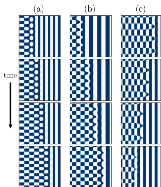
Figure 4.5: Snapshots of the dynamics of fronts that separate stripe and rectangular patterns. Lower energy patterns invade the regions of higher energy patterns: (a) rectangular pattern invading 1 : 1 stripes ( k_f/k_0 = 1.10 ), (b) rectangular pattern invading 2 : 1 stripes ( k_f/k_0 = 1.65 ), and (c) 2 : 1 stripes invading a rectangular pattern ( k_f/k_0 = 1.80 ). The domain sizes of simulations (a), (b) and (c) are 50 \times 50 , 60 \times 60 and 50 \times 50 , respectively. Parameters: \epsilon = 0.1 , \gamma = 0.4 .
