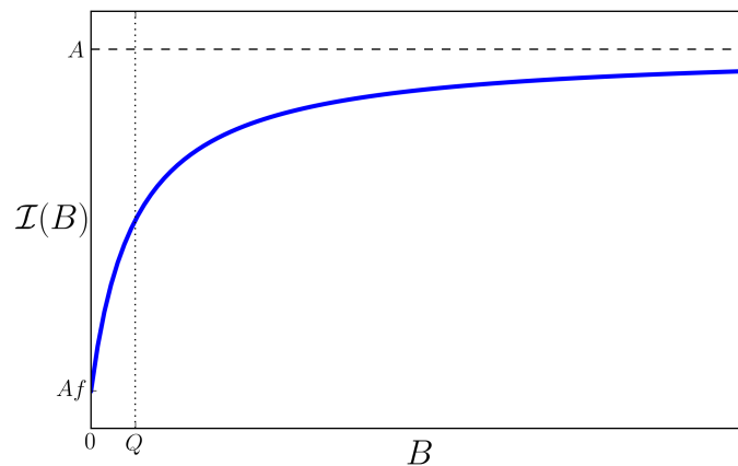
Figure 2.8: The infiltration as a function of the biomass.
