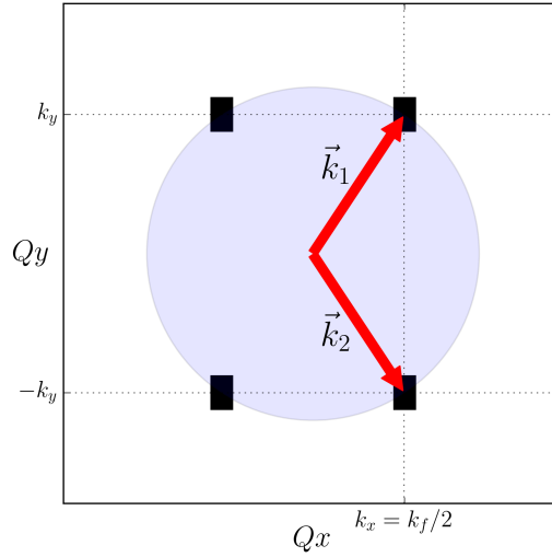
Figure 2.7: Fourier transform of the rectangular pattern shown in Figure 2.6. The two vectors in red have coordinates \vec{k}_1 = (k_x, k_y) and \vec{k}_2 = (k_x, -k_y) . The circle in blue has radius k_0 .
