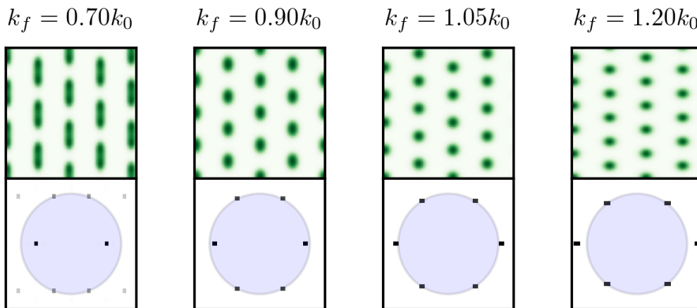
Figure 5.16: Four rectangular patterns calculated for different values of forcing wavenumber. The upper panels show the biomass on a 200 \times 200 domain, and the lower panels depict the Fourier transform. The four wavevectors responsible for the rectangular pattern always sit on the border of the blue circle, whose radius is k_0 = 0.143 , while the two strong wavevectors \mathbf{k} = \pm k_f \hat{x} can be found either inside or outside it. Parameters: p = 0.80 , \gamma_f = 1.0 .
