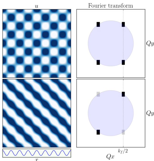
Figure 2.6: Two dimensional solutions of Equation (2.8). On the top left a rectangular pattern ( \gamma = 0.2 ), and below it an oblique pattern ( \gamma = 0.05 ). The panels on the right show the patterns' respective Fourier transform absolute value, where the circle in blue has radius k_0 . The short box on the lower left indicates the periodic forcing in x . Parameters: \epsilon = 0.1 , k_f = 1.1 , k_0 = 1.0 .
